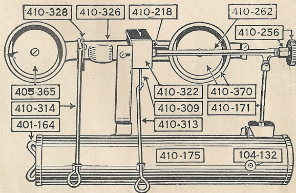
Gypsy Camp Stove No. 10
