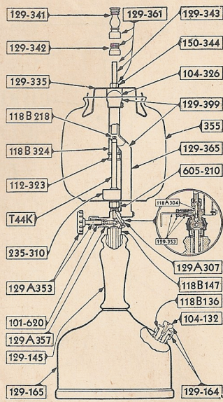
Kerosene Mantle Lamp Alcohol Generating Lamp No. 129
