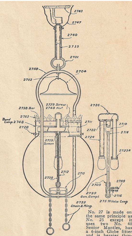
Ceiling Fixture System Lamp No. 27
