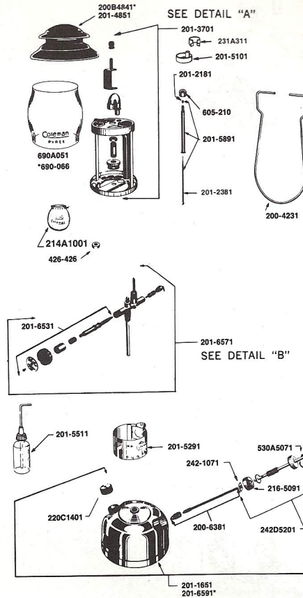
MODEL 201-700 SHOWN
